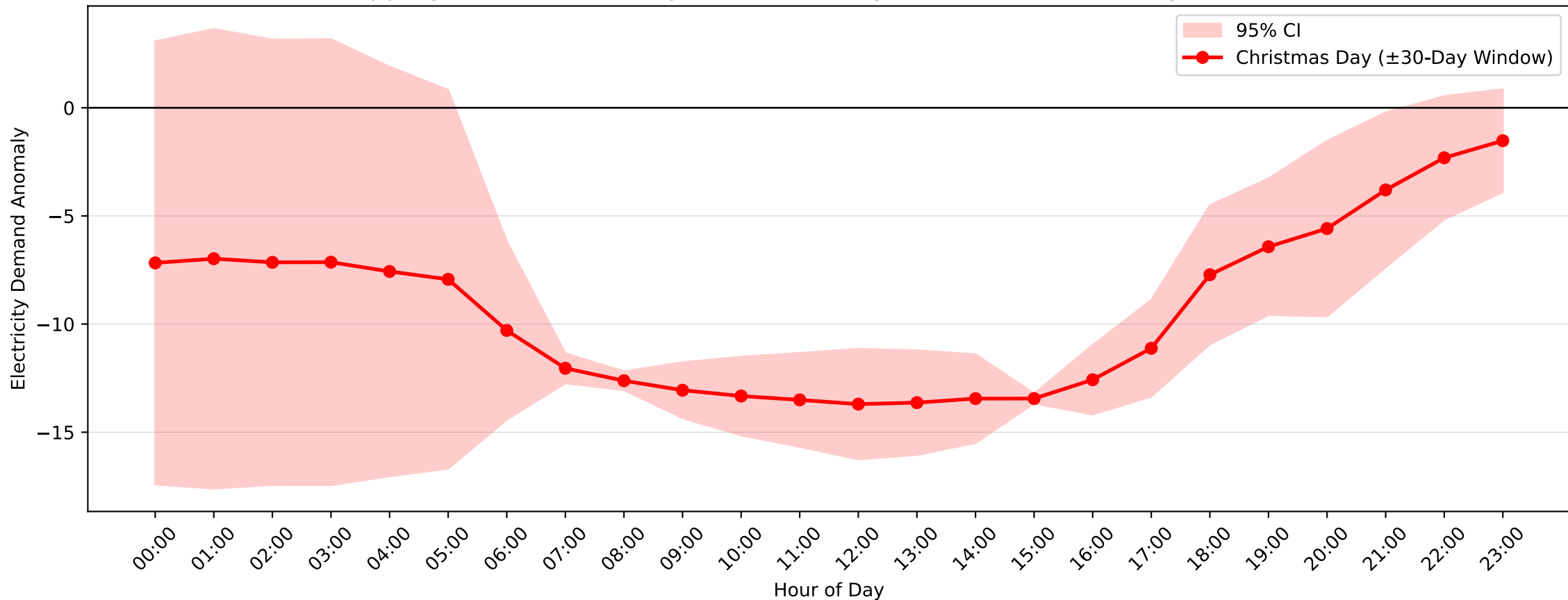
Epping Demand Anomaly: Christmas Day (2009–2010, \pm 30 -Day Window)
