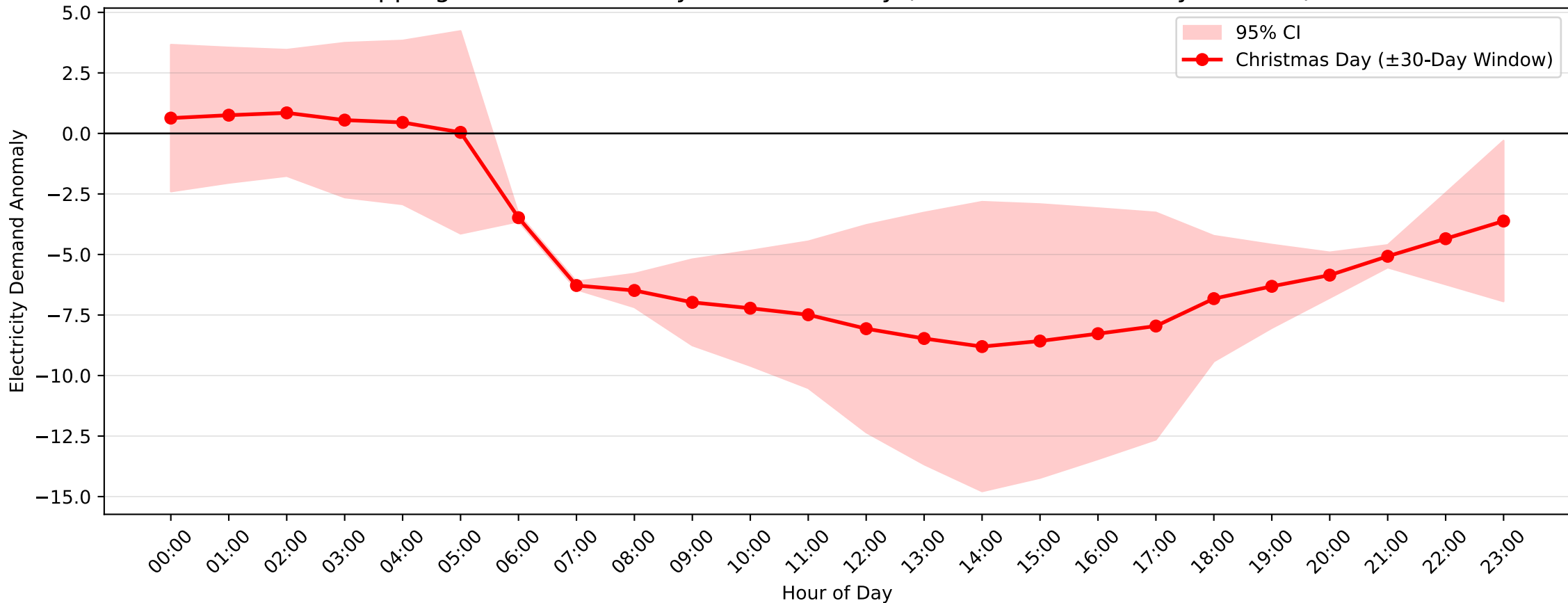
Epping Demand Anomaly: Christmas Day (2014–2015, \pm 30 -Day Window)
