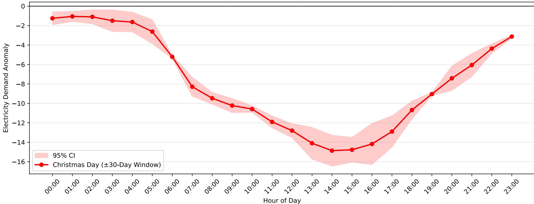
Epping Demand Anomaly: Christmas Day (2007-2008, \pm 30 -Day Window)
