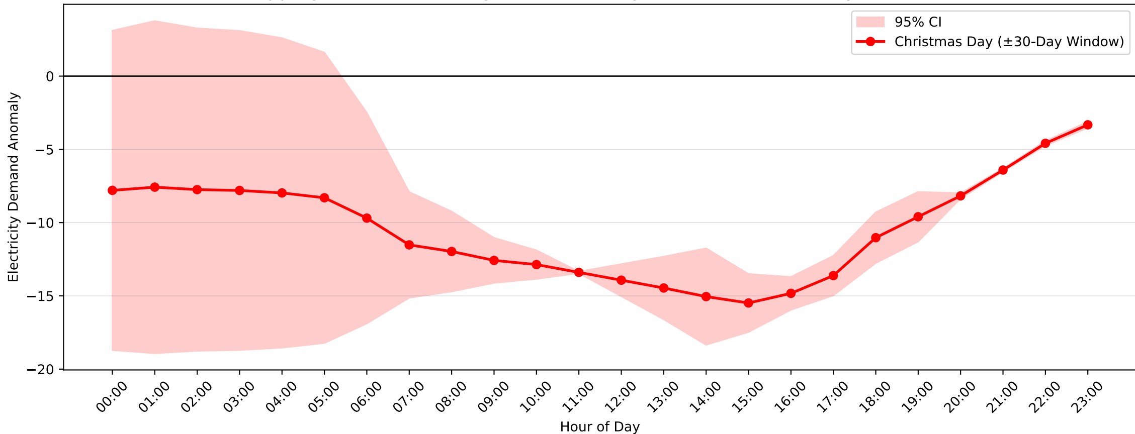
Epping Demand Anomaly: Christmas Day (2008-2009, \pm 30 -Day Window)
